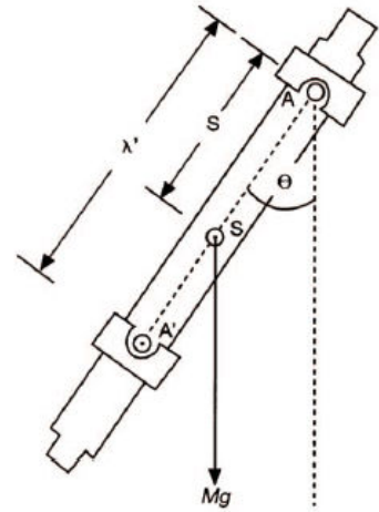
Fig. 1: Reversible pendulum.
